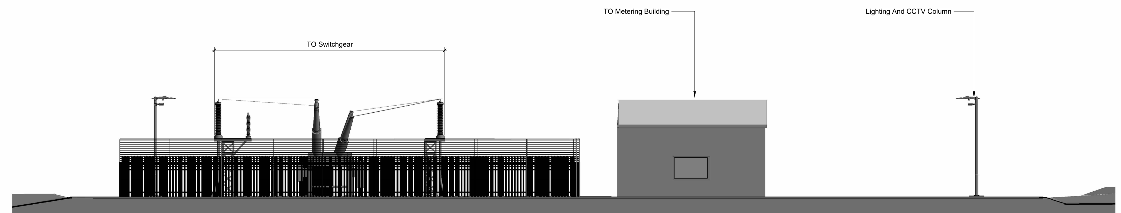
4 NORTH-WESTERN ELEVATION 1:100
