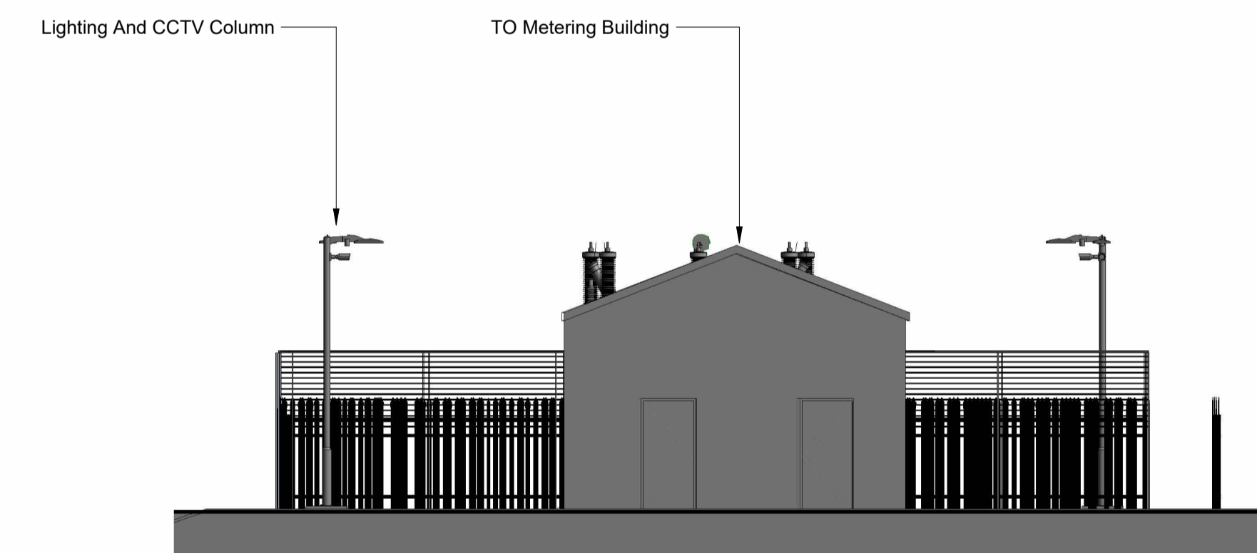
3 SOUTH-WESTERN ELEVATION 1:100
